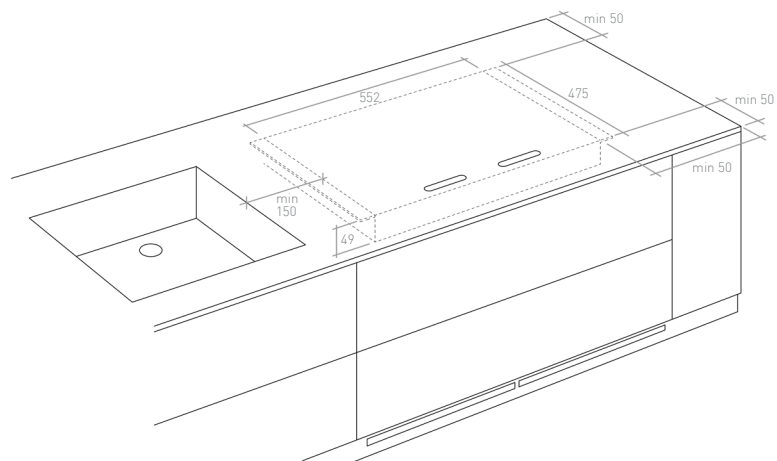
Img 1: Induction unit dimensions and minimum distances from the edges (50mm) and holes (150mm) of the worktop.
