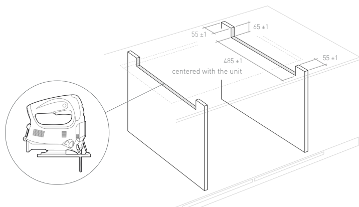
Img 2: Shape the sides of the base if it is not possible to maintain the recommended distances in Img. 3.
